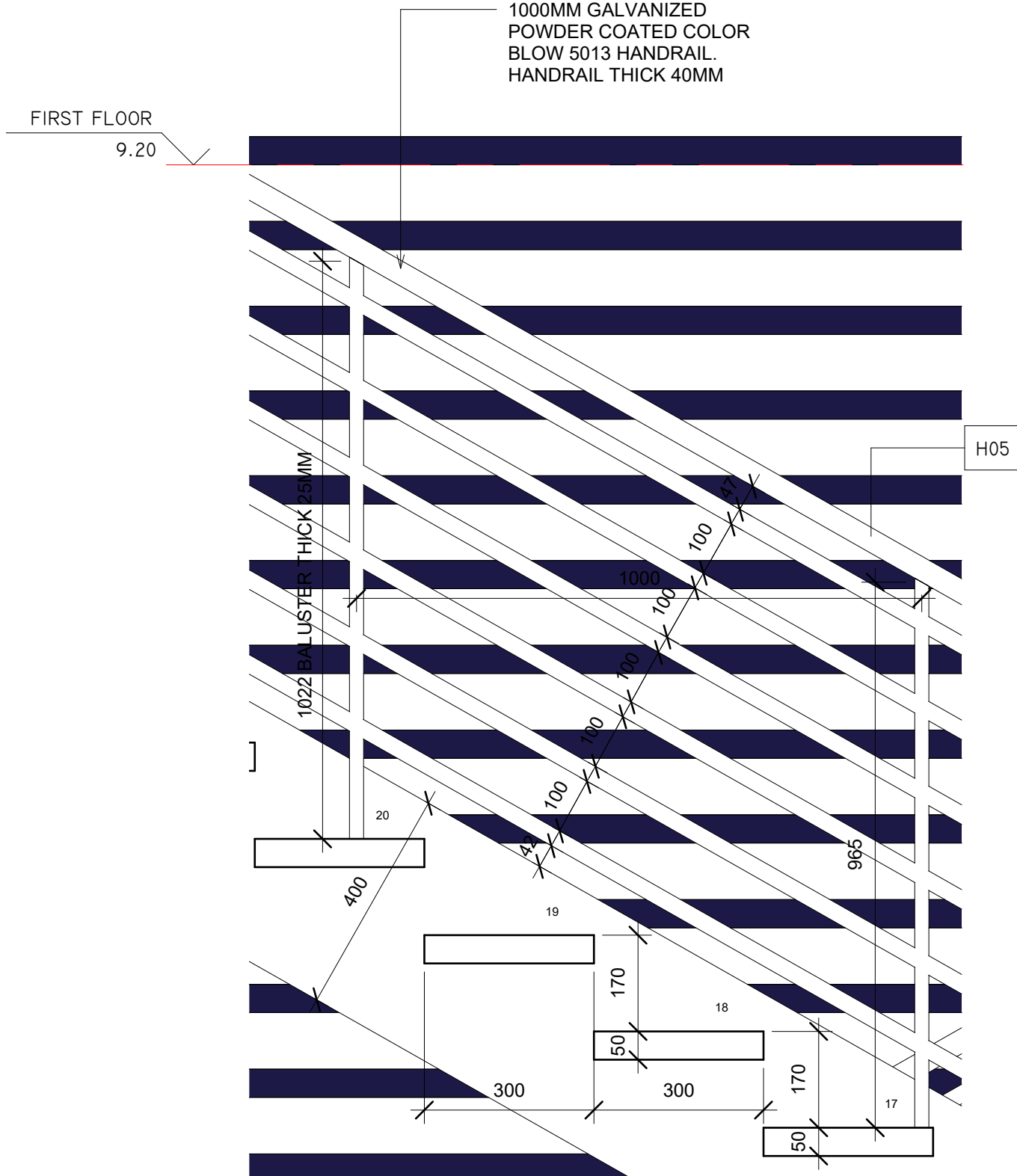
4 SECTION-I (STAIRCASE -I) - CALLOUT I 1 : 10
